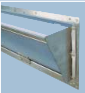
Fold-out side shields direct air and increase air flow velocity through inlet.
